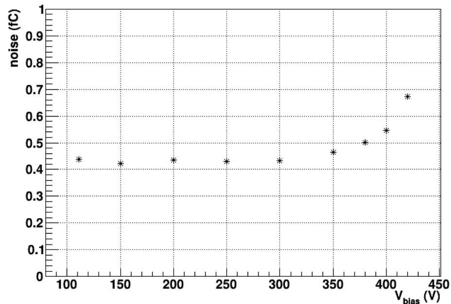
USTC-IME_W24-P23_1x2-LGAD-far_15e14
