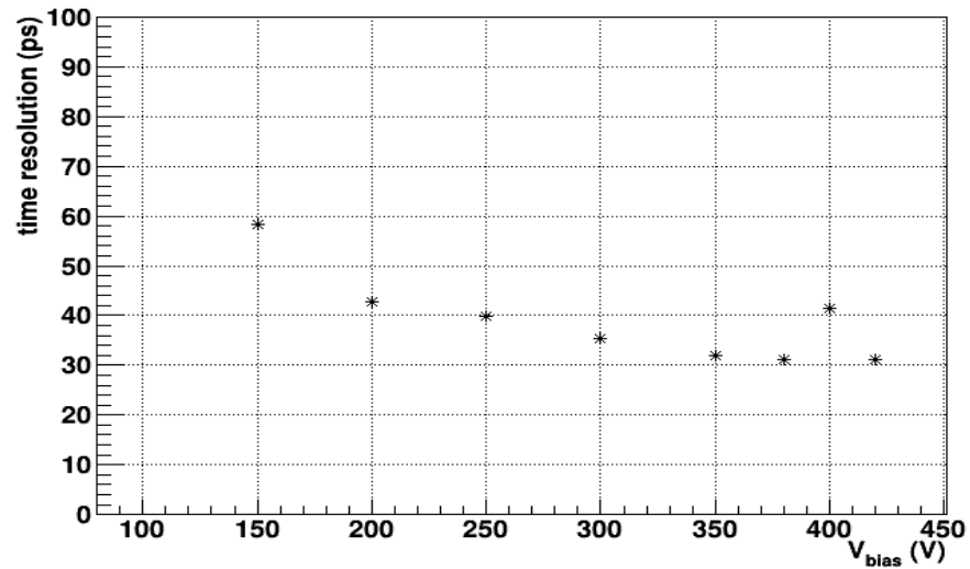
USTC-IME_W24-P23_1x2-LGAD-far_15e14
