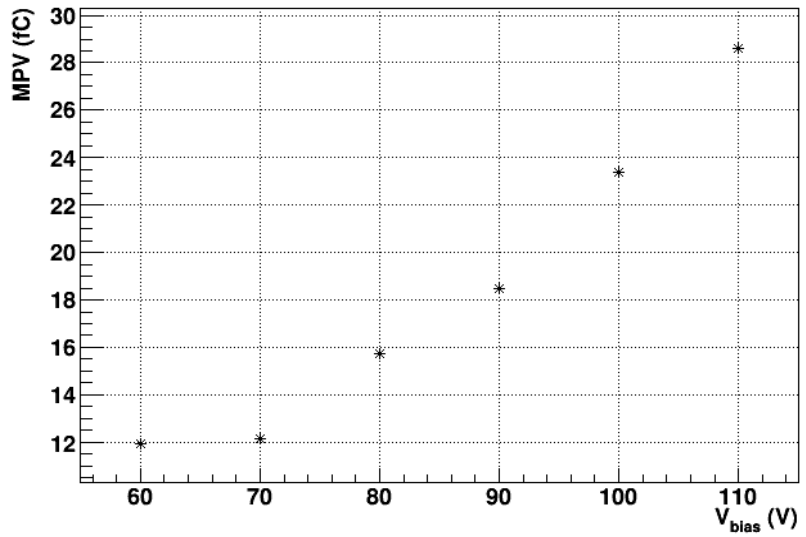
IHEP-IME_V1R2-20-1x1_0e14
