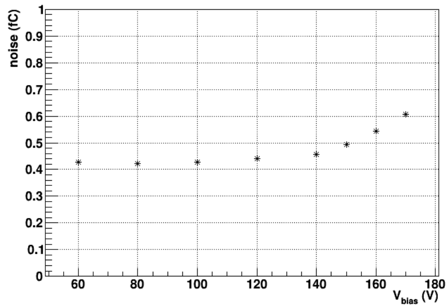
USTC-IME_W24-P29_1x2-LGAD-far_4e14
