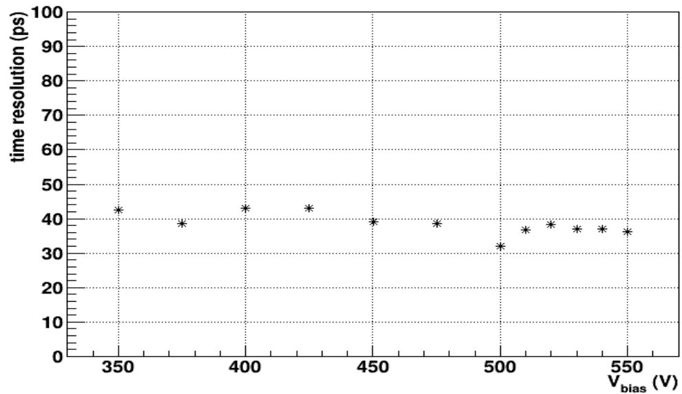
IHEP-IME_V1R2-31-1x2-LGAD2_25e14
