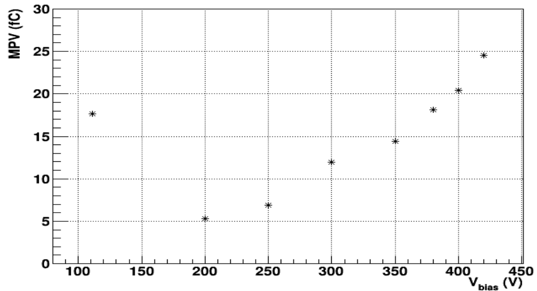
USTC-IME_W24-P23_1x2-LGAD-far_15e14
