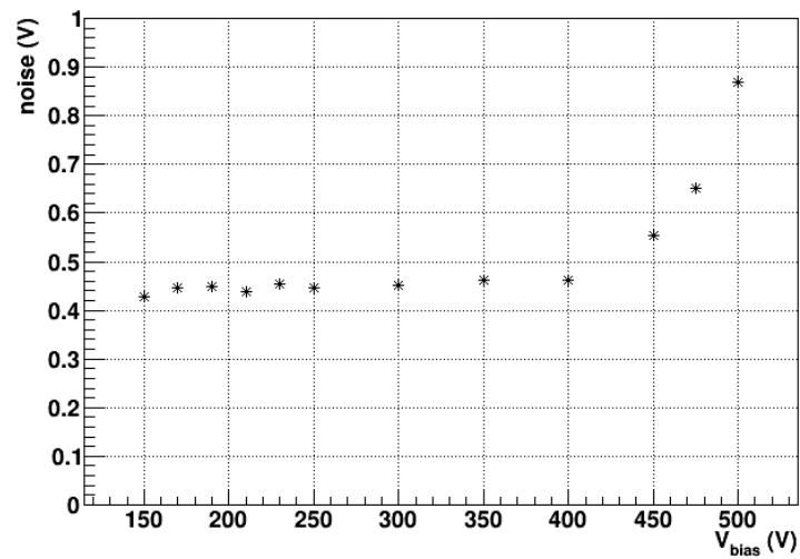
IHEP-IME_V1R2-24-1x2-LGAD2_15e14
