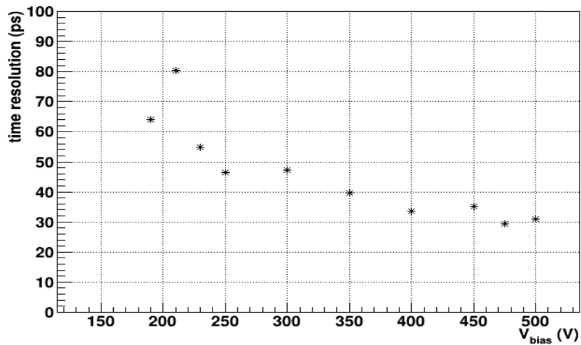
IHEP-IME_V1R2-24-1x2-LGAD2_15e14
