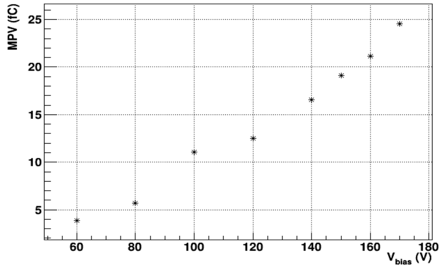
USTC-IME_W24-P29_1x2-LGAD-far_4e14
