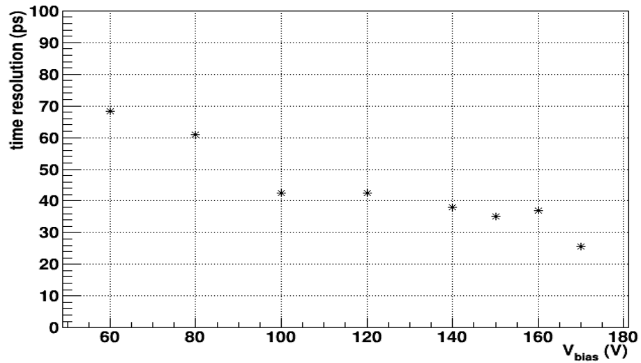
USTC-IME_W24-P29_1x2-LGAD-far_4e14
