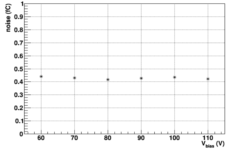
IHEP-IME_V1R2-20-1x1_0e14
