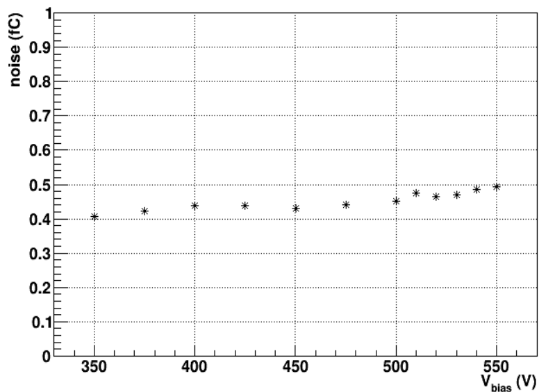
IHEP-IME_V1R2-31-1x2-LGAD2_25e14
