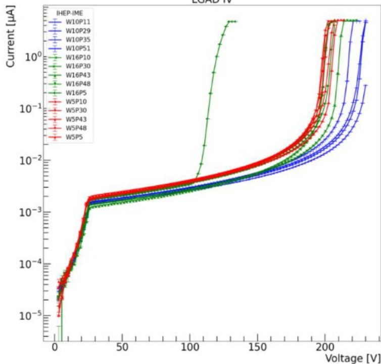
LGAD IV
