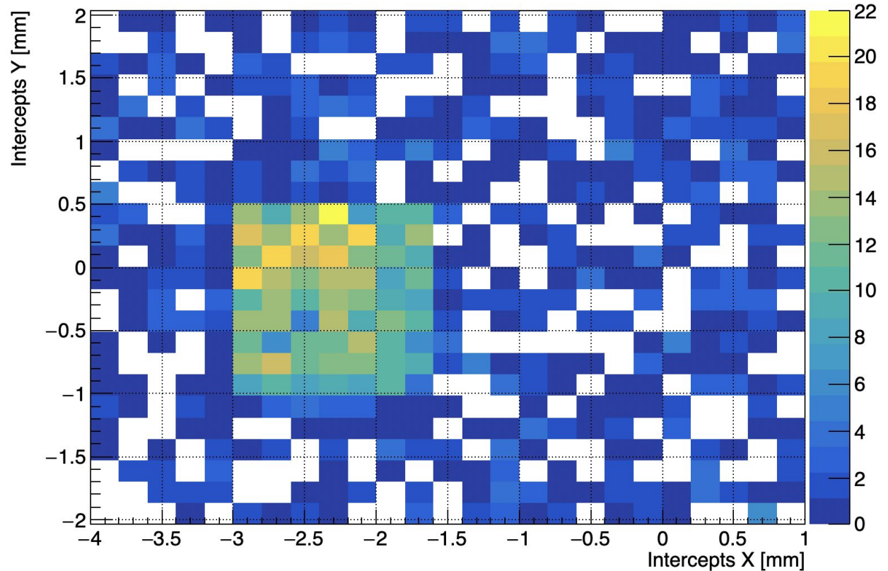
Track Intercepts in DUT
