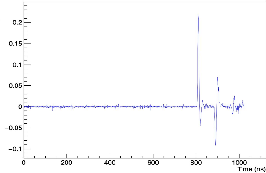
Collected Charge vs Time for Event 0
