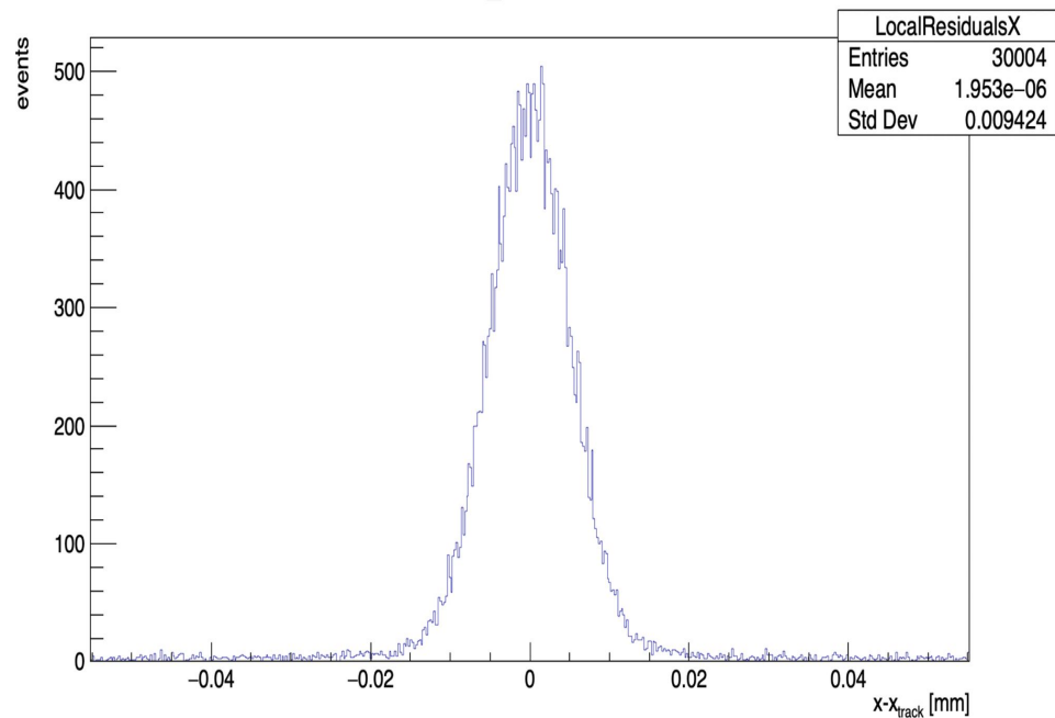
MIMOSA26_3Local Residual X
