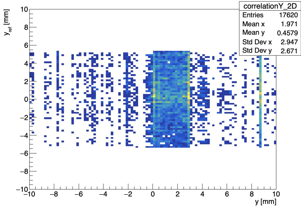
RD53B_115: 2D correlation Y (global)
