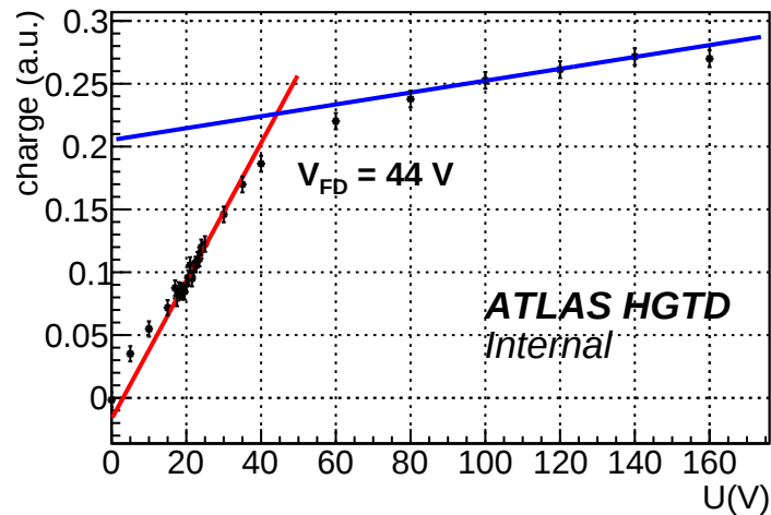
GAP signal
