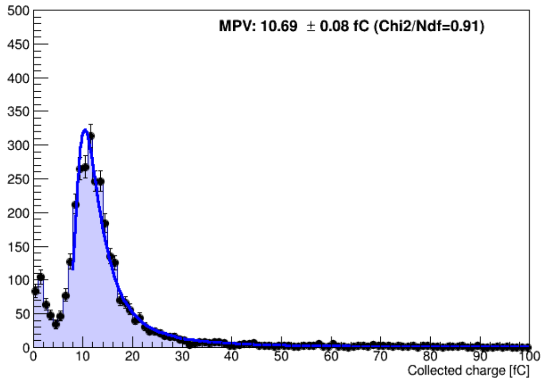
Pixel (6, 6) collected charge distribution
