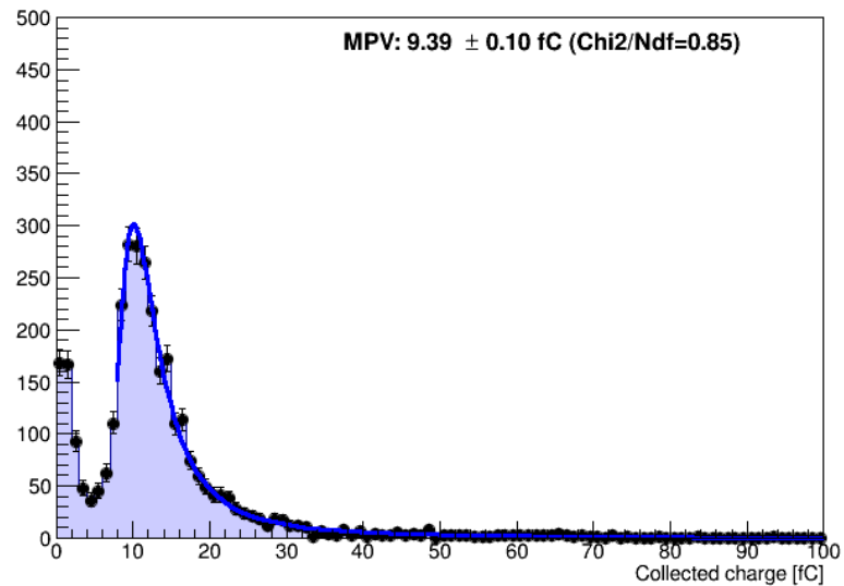
Pixel (7, 6) collected charge distribution
